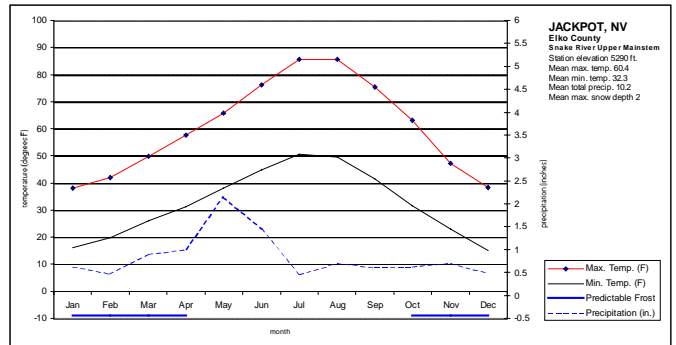
Figure A-1. Summary of climatic patterns with the Snake River Upper Mainstem Subbasin. Mean monthly and annual climatic data are summarized for selected weather stations within the subbasin. Stations are selected to represent broad climatic regimes. The distribution of climatic regimes within the subbasin is displayed in the upper left corner. See Table 3.3 for detailed descriptions of the Koppen climatic classes.
